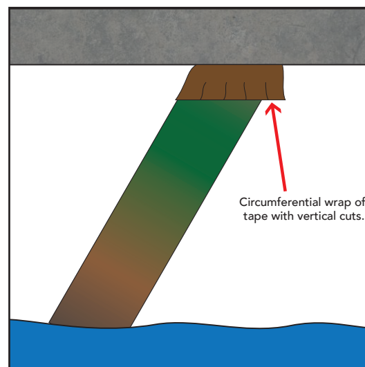
Fig. 1: Application of the Marine Piling Tape.
