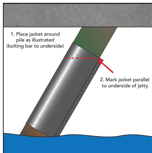
Fig. 4: How to locate and mark the HDPE Jacket for cutting.
