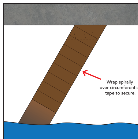
Fig. 3: Circumferential wrap of Marine Piling Tape.
