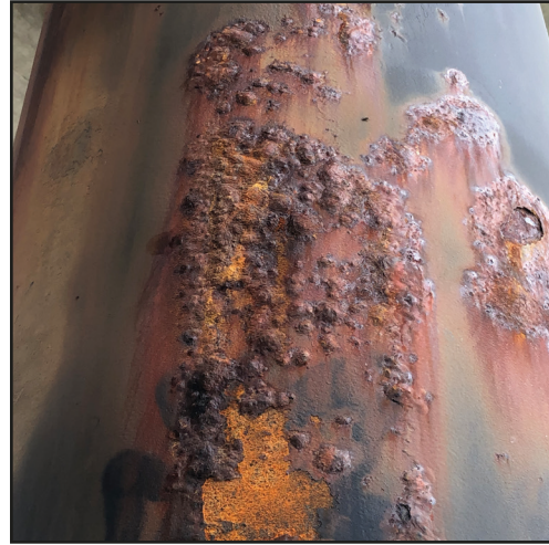
Example image of a pile featuring a loosely adhering corrosion prevention coating that would require removal.
