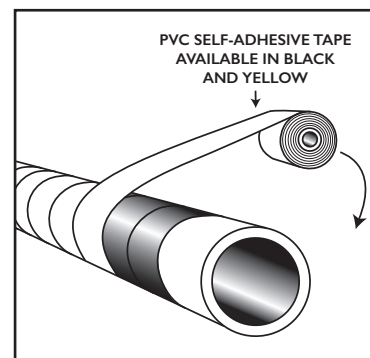
Fig. 10: An additional layer of Denso PVC Self-Adhesive Tape can be added for extra mechanical protection over the inner layer of Densopol. Please consult with the manufacturer for advice.
